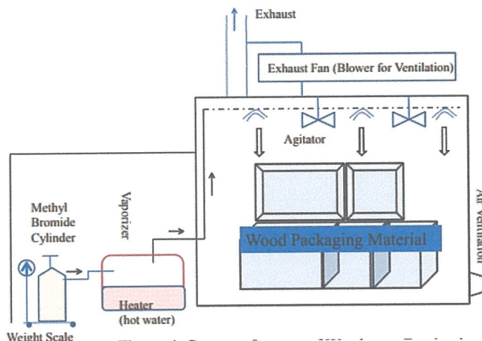
Figure Q4: Common layout of warehouse fumigation
