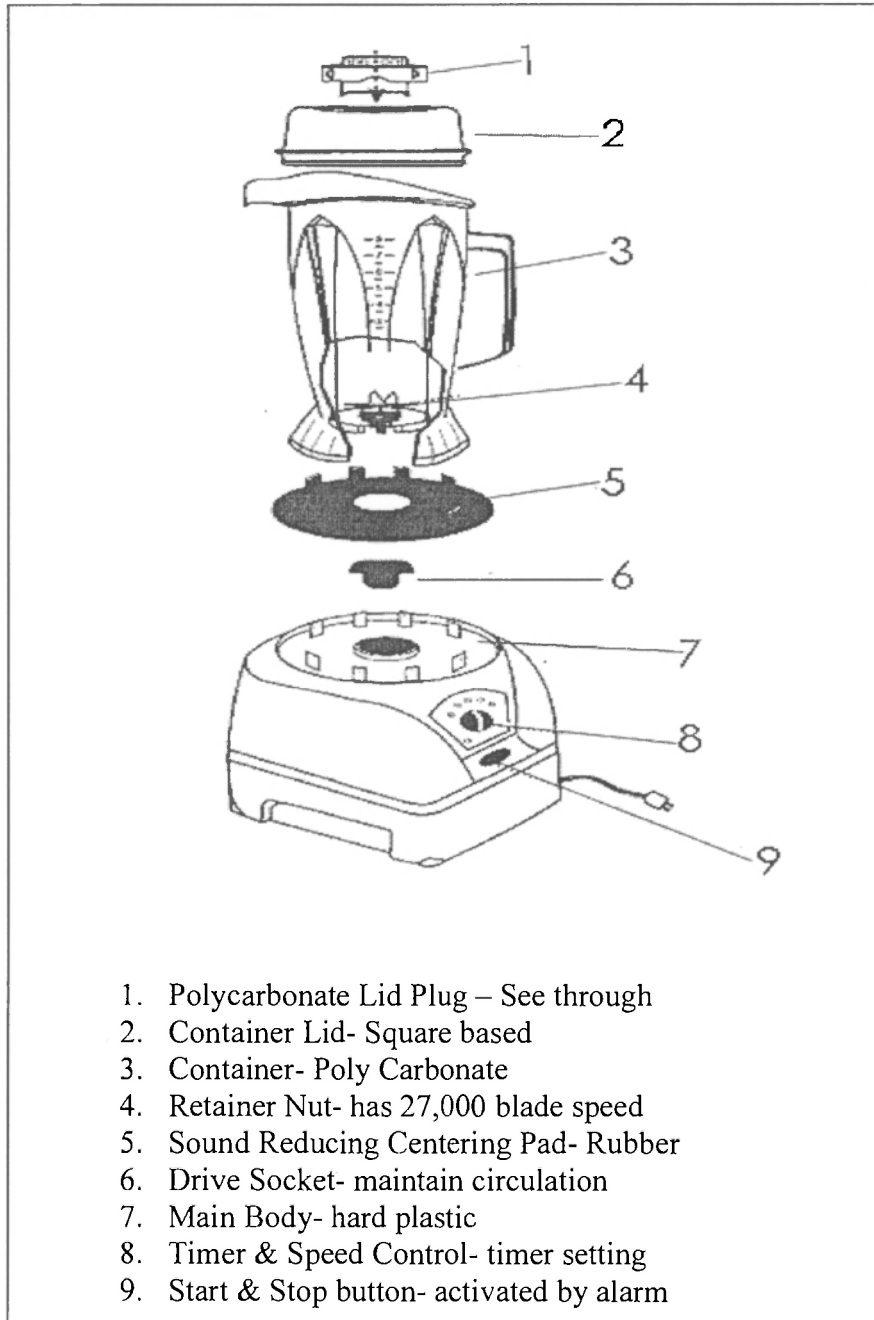
Figure 1: Food processor
