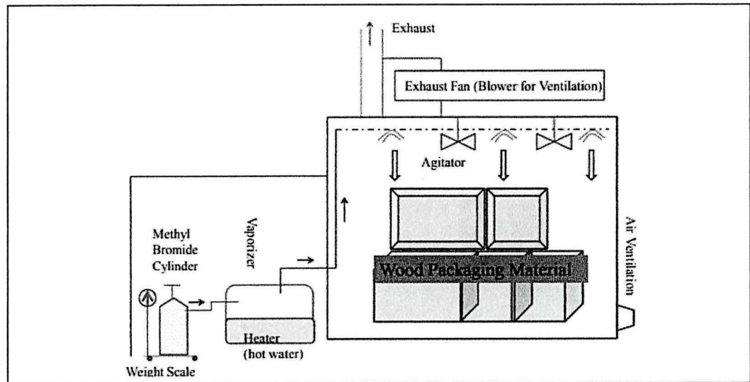
Figure Q4: Common layout of warehouse fumigation
